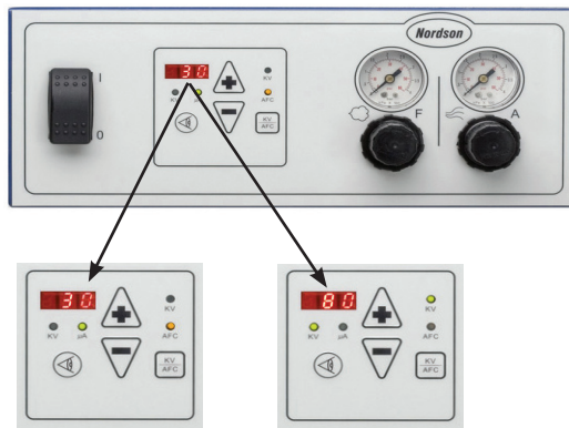
The Vantage controller features dual-mode operation to monitor current and voltage for greater flexibility.
